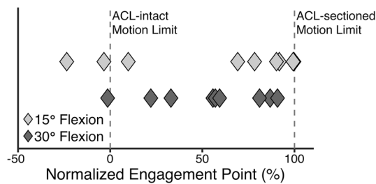
Fig. 5 Normalized engagement points of the ALL in response to combined valgus and internal rotation torques are shown individually for each knee that was tested. Light and dark gray diamonds represent the normalized engagement point of the ALL in each knee at 15° and 30° of flexion, respectively. The engagement points are expressed as a percentage of the difference between the ACL-intact and -sectioned motion limits (dashed gray lines) in the same knee. A negative percentage indicates engagement within the ACL-intact motion limit.
